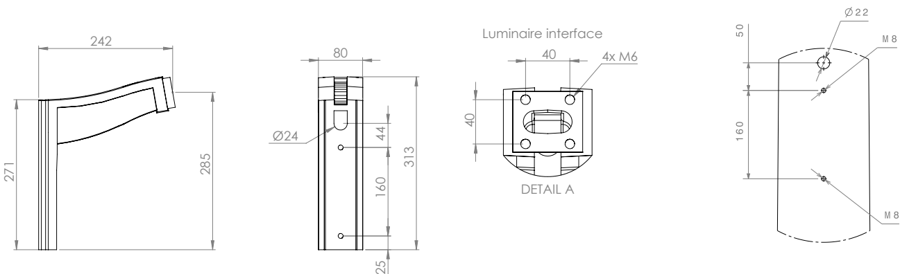
Drilling information (for lateral mounting on pole)
