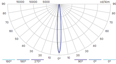
5124 RGB+CW (all ON 100%) Narrow Beam, No diffuser
